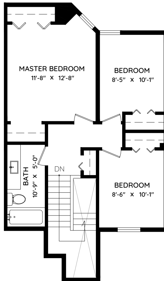
UPPER FLOOR 578 SQ.FT. CH: 8'-0"
